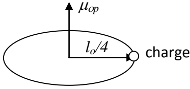
Fig. 4. Definition of the Planck scale magnetic moment for the proton.
