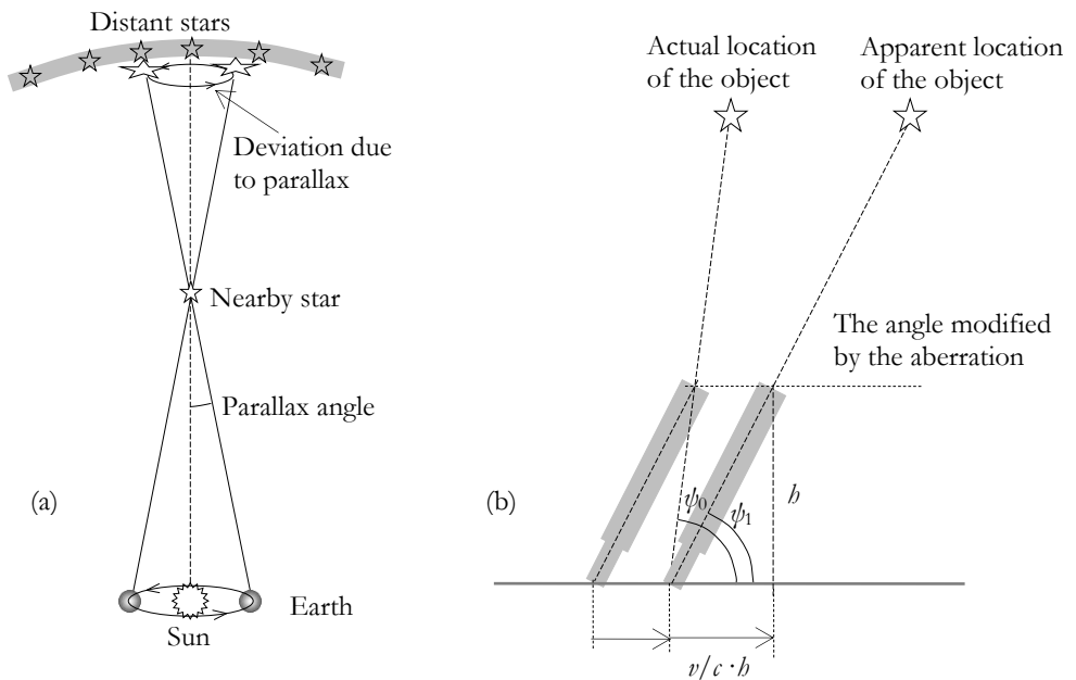
Figure 1-11. (a) If the Earth is assumed to revolve around the Sun, one should expect that the apparent position of nearby stars against distant stars should change during the year due to the parallax. The detection of the parallax was not possible with Tycho Brahe's instruments. (b) In the measurement of the angle of the object, due to aberration, the velocity of the observer gives rise to an apparent deviation from the actual observation angle. If the telescope used has the velocity v in the direction of the object at the observation plane, the telescope must be tilted to the angle \psi_1 , in order to let the light entering to the top of the telescope reach the observer's eye at the lower end. The mechanism of aberration was first explained by the English astronomer James Bradley in the 18 th century.
