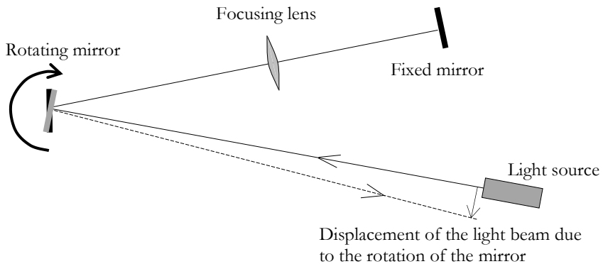
Figure 1-22 Apparatus used by Léon Foucault and Hippolyte Fizeau for the determination of the velocity of light in 1850. Albert Michelson's apparatus, in 1883, applied the same principle of operation. He obtained the value of 299,864 \pm 51 km/s for the velocity of light.
