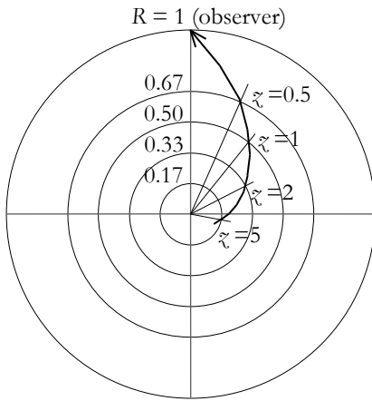
Figure 3-16. The length of the R_0 radius and the location of objects for redshifts z = 0 to 5. Location R_4 = 1 is the observer's location. The optical distance to the object is the tangential length of the path, which is equal to the difference between the current R_4 radius and the R_{4(0)} radius as it was when the light was emitted. For example, the light emitted at R_4 = 0.17 in the drawing is redshifted by z = 5 after traveling the distance D = (1-0.17)R_0 in expanding space.
