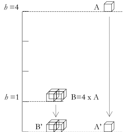
Figure 1-14. Leibniz's experiment for the determination of vis viva .
