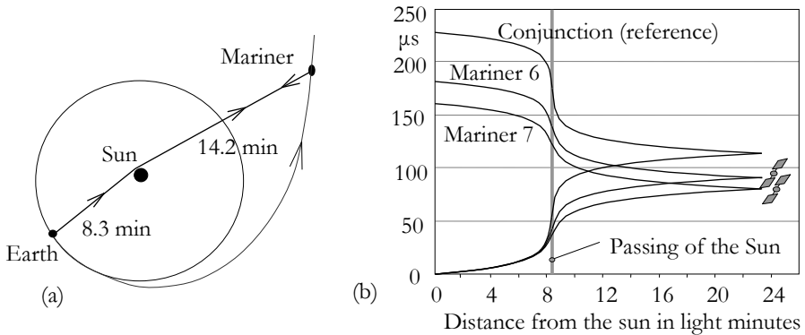
Figure 3-21. (a) Measurement of the delay in a radio signal due to the gravitation of the Sun. (a) The route of the Mariner space crafts from the Eart to Mars and the path of the radio signal to and from Earth. (b) The development of the two-way radio signal passing the Sun in Mariner 6 and Mariner 7 experiments.
